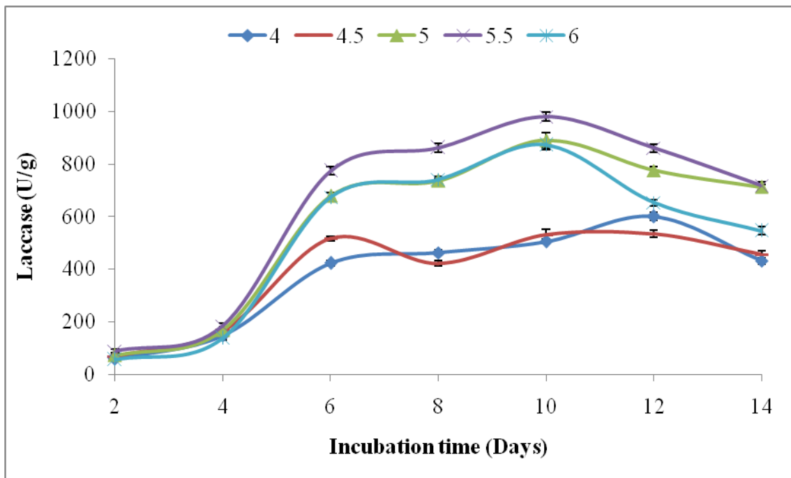
Fig. 3 Effect of pH on laccase production
