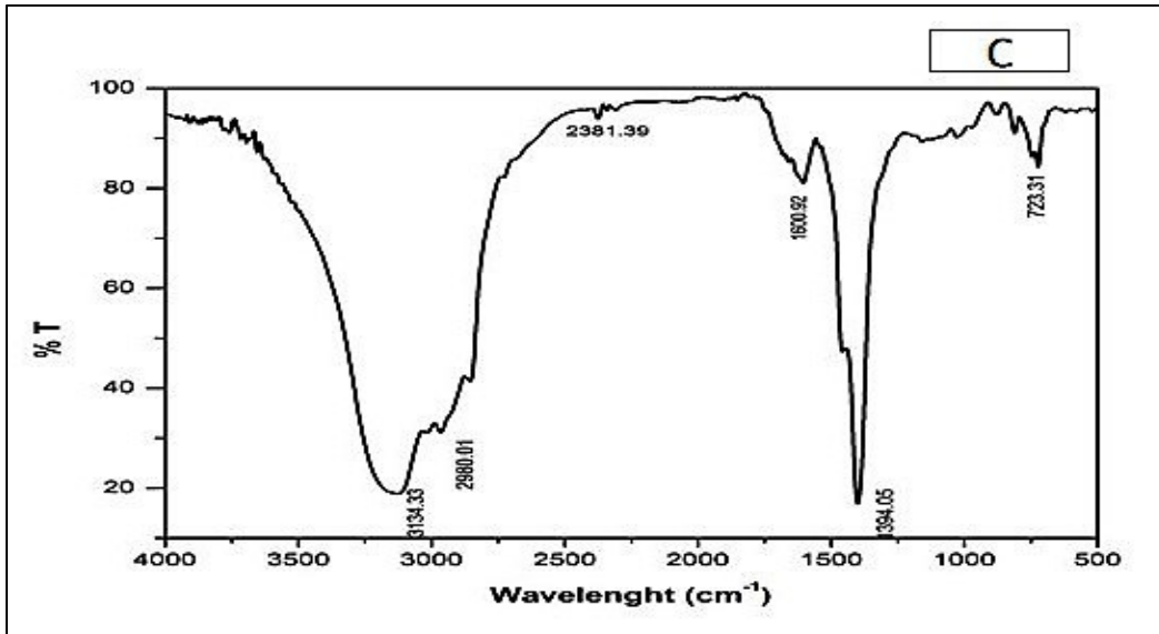
Fig.1. FTIR spectra of crude oil (untreated control sample)
