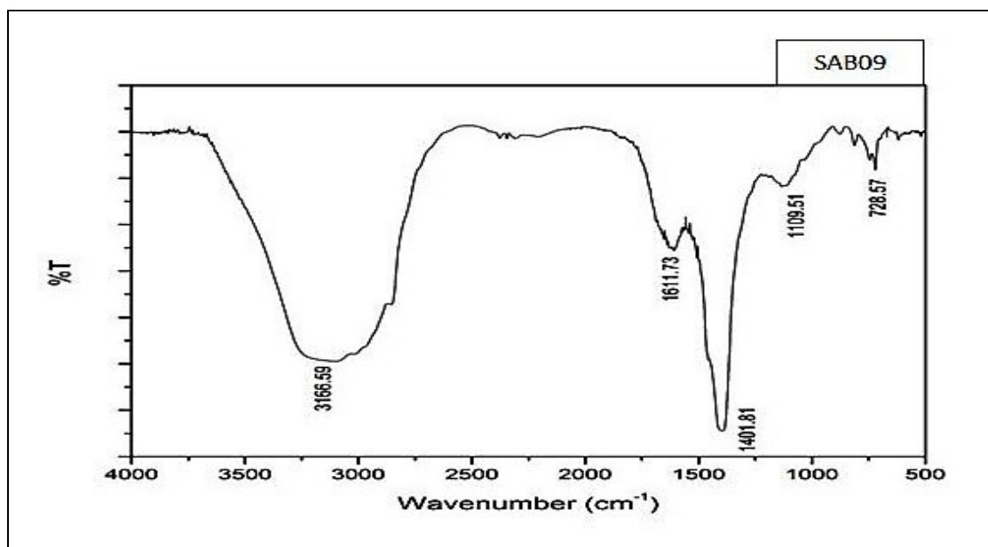
Fig.3. FTIR spectra of crude oil extracted after treatment with isolate SAB09
