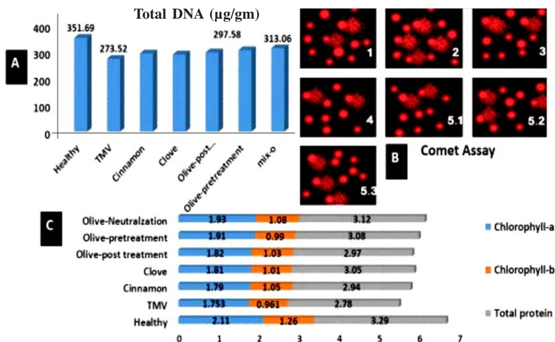
Fig. 4. Total DNA, A; numerical measurements by Comet Assay and Genotoxicity measuring the damages in the DNA using Tail Moment in Datura plants for all treatments. B; and Total Protein Content and Chlorophyll. C as a physiological responses to the treatments with essential oils against Virus in chlorophylls and the Protein in Mg/gm.
