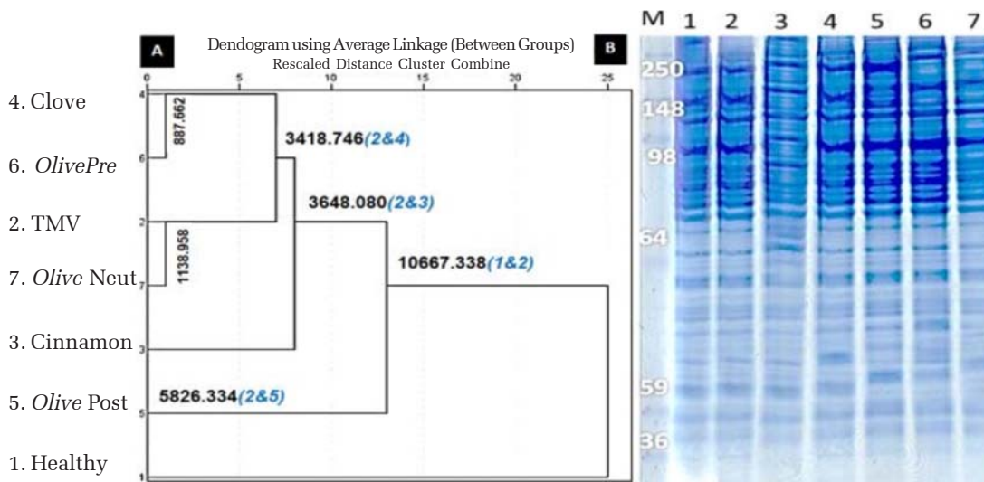
Fig. 6. PAGE Analysis A and B of the treated Datura leaves by different tested essential oils using dendrogram by average linkage, between groups, rescaled distance cluster combine
