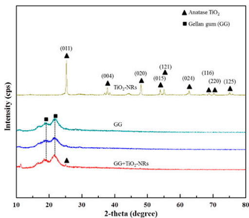
Fig. 4. XRD diffractogram of \text{TiO}_2 -NRs, GG, and GG+ \text{TiO}_2 -NRs films
