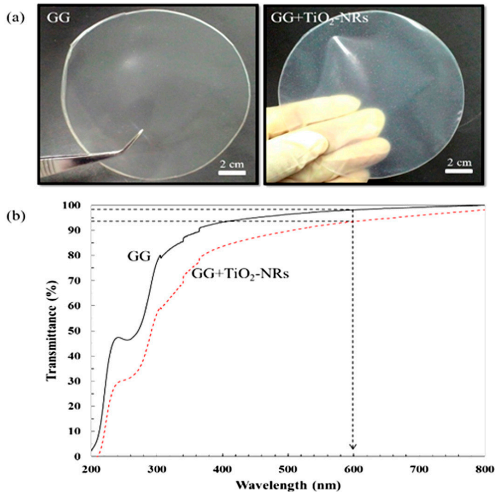
Fig. 1. (a) Physical appearance of GG and GG+TiO 2 -NRs (b) UV-Vis transmittance of GG and GG+TiO 2 -NRs films
