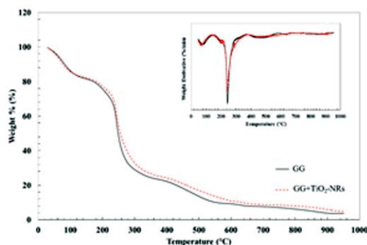
Fig. 5. TGA thermogram of GG and GG+ \text{TiO}_2 -NRs films
