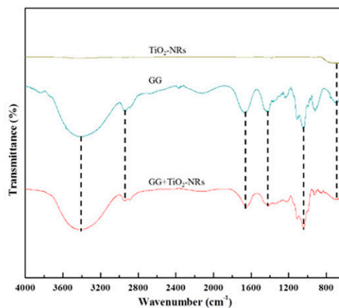
Fig. 3. FTIR spectra of TiO 2 -NRs, GG, and GG+TiO 2 -NRs films
