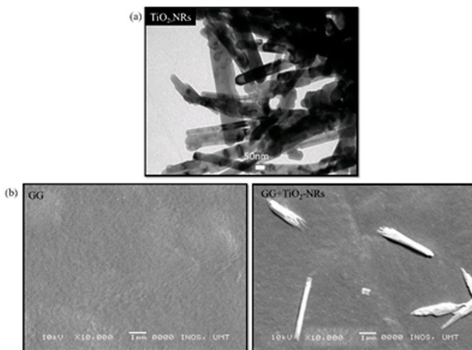
Fig. 2. (a) TEM micrographs of TiO 2 -NRs (b) SEM micrographs of GG and GG+TiO 2 -NRs films
