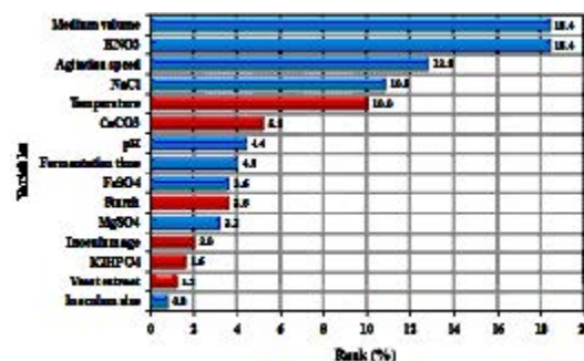
Fig. 4. Pareto chart illustrates the order of significance of the variables affecting the bioactive metabolites production, Ranks (%) values ranging from 0.80 to 18.4
