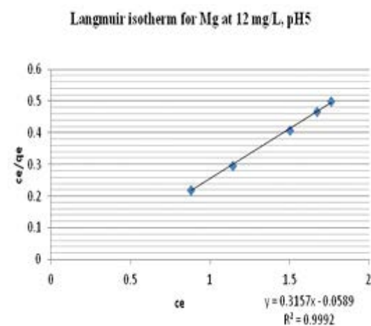
Fig. 6. Langmuir isotherm for magnesium
