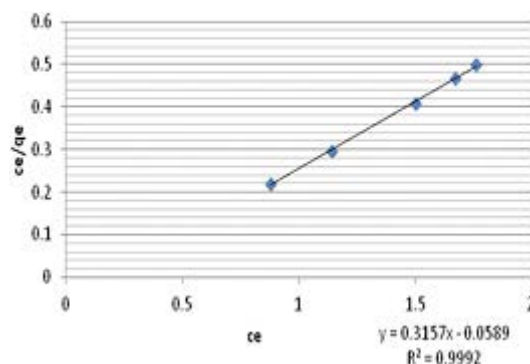
Fig. 7. Langmuir isotherm for lead
