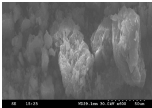
Fig. 4. CTLR after treatment with electroplating effluent
