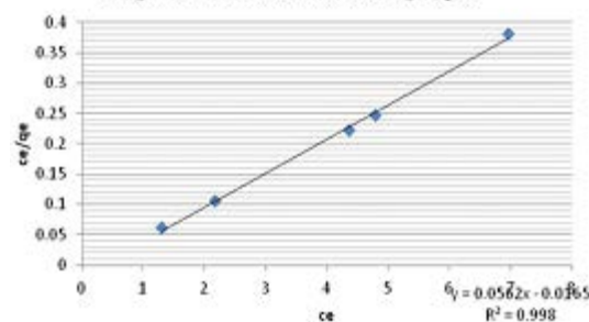
Fig. 8. Langmuir isotherm for chromium
