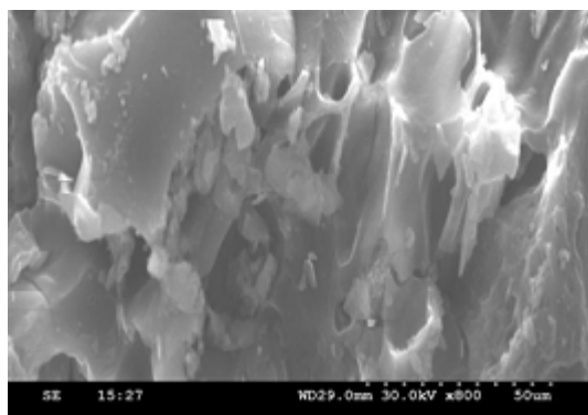
Fig. 3. CTLR before treatment with electroplating effluent
