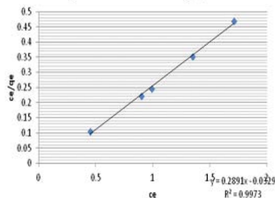
Fig. 9. Langmuir isotherm for zinc
