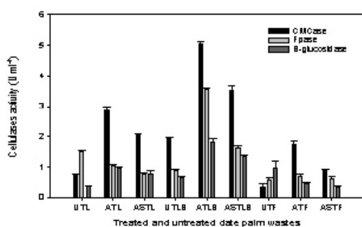
Fig. 3. Cellulase production by Geobacillus stearothermophilus using treated and untreated date palm waste as carbon sources (UTL: Untreated leaves, ATL: Alkaline treated leaves, ASTL: Acid-steam treated leaves, UTLB: Untreated leaf base, ATLB: Alkaline treated leaf base, ASTLB: Acid-steam treated leaf base, UTF: Untreated fibrous, ATF: Alkaline treated fibrous, ASTF: Acid-steam treated fibrous).
