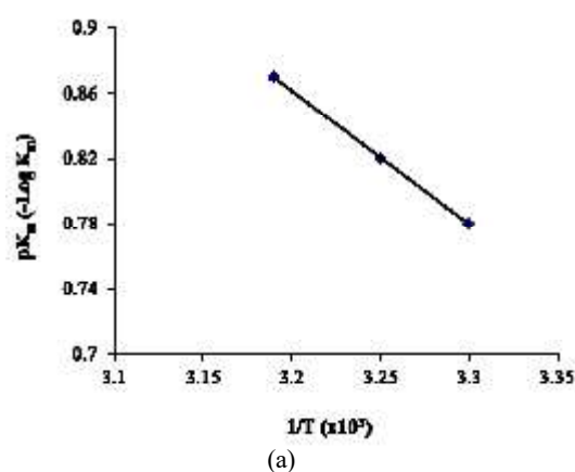
Fig. 8. Effect of temperature on K_m and V_{max} of purified lipase from P. aeruginosa
