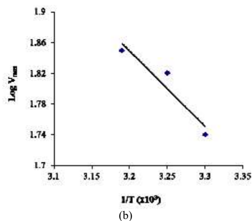
Fig. 8. Effect of temperature on K_m and V_{max} of purified lipase from P. aeruginosa
