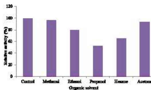
Fig. 6. Effect of different organic solvents on the activity of purified lipase from P. aeruginosa
