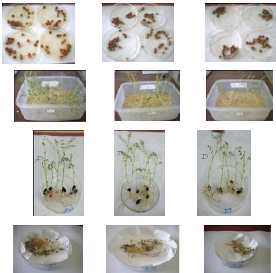
Fig. 2. Chick pea seed treatment process (A) showing the seed treatment process of Fig1b: Uprooted cicer aritenum plants Cicer aritenum seeds and their growth in crystal sand (B) Uprooted cicer aritenum plants and (C) Dried Cicer aritenum plants
