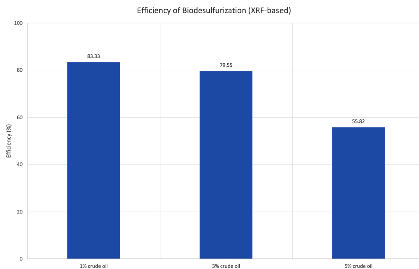
Figure 5. Biodesulfurization Efficiency
