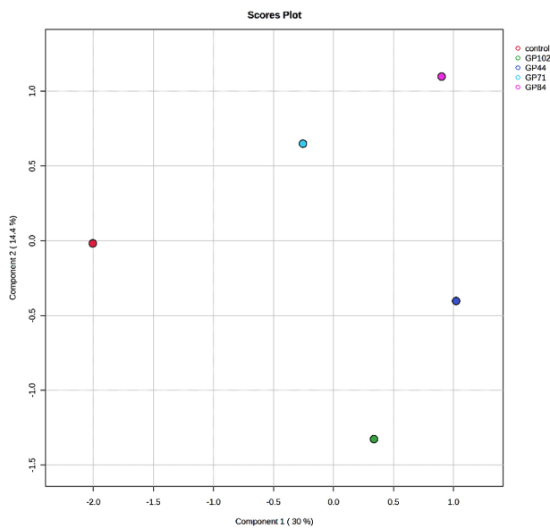
Figure 1b. Partial Least Squares-Discriminant Analysis (PLS-DA) of the VOCs detected in the uninoculated control and garden pea root nodule isolates
