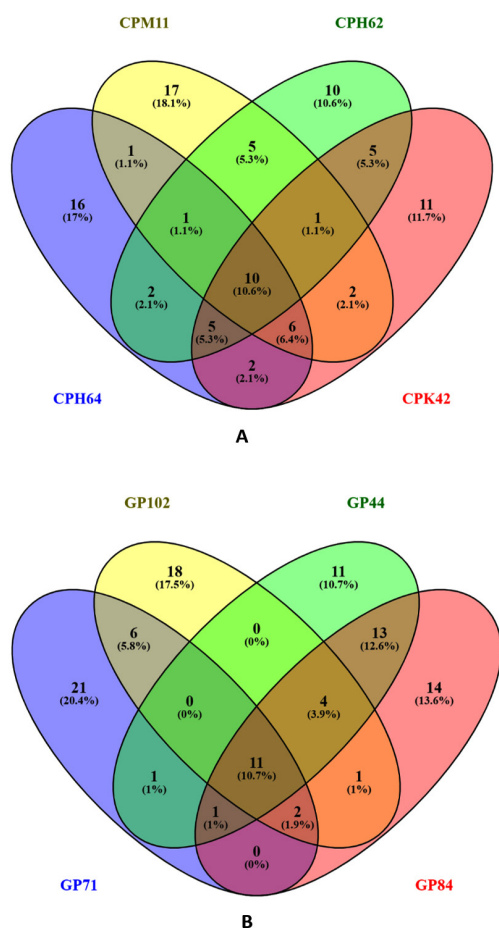
Figure 2. Venn diagram displaying the number of volatile organic compounds coincident between the bacterial strains isolated from (A) cowpea and (B) garden pea root nodules
