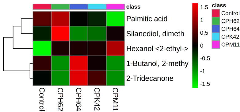
Figure 3. Heatmap of the VOCs with putative plant growth promotion abilities produced by bacterial isolates obtained from cowpea nodules. The columns represent the bacterial isolates, and the rows represent the different metabolites identified. The colour codes indicate the abundance of each VOC
