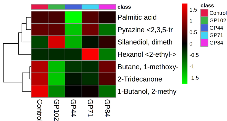
Figure 4. Heatmap of the VOCs with putative plant growth promotion abilities produced by bacterial isolates obtained from garden pea nodules. The columns represent the bacterial isolates, and the rows represent the VOC's identified. The colour codes indicate the abundance of each VOC
