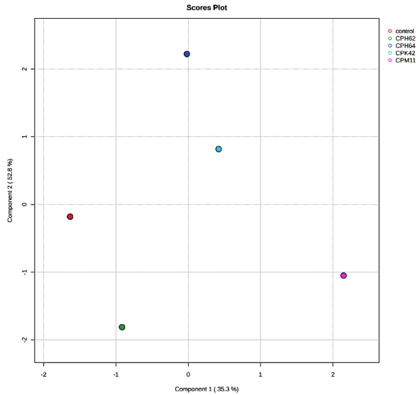
Figure 1a. Partial Least Squares-Discriminant Analysis (PLS-DA) of the VOCs detected in the uninoculated control and cowpea nodule isolates
